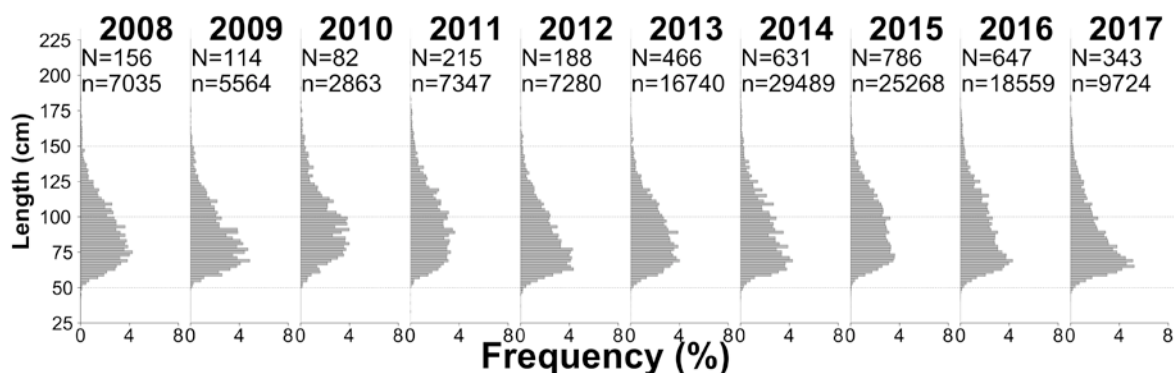
Figure 1: Annual length-frequency distributions of Dissostichus eleginoides caught in the South African EEZ from 2008 to 2017. The number of hauls from which fish were measured (N) and the number of fish measured (n) in each year are provided. (Note: data for 2017 are incomplete.)
